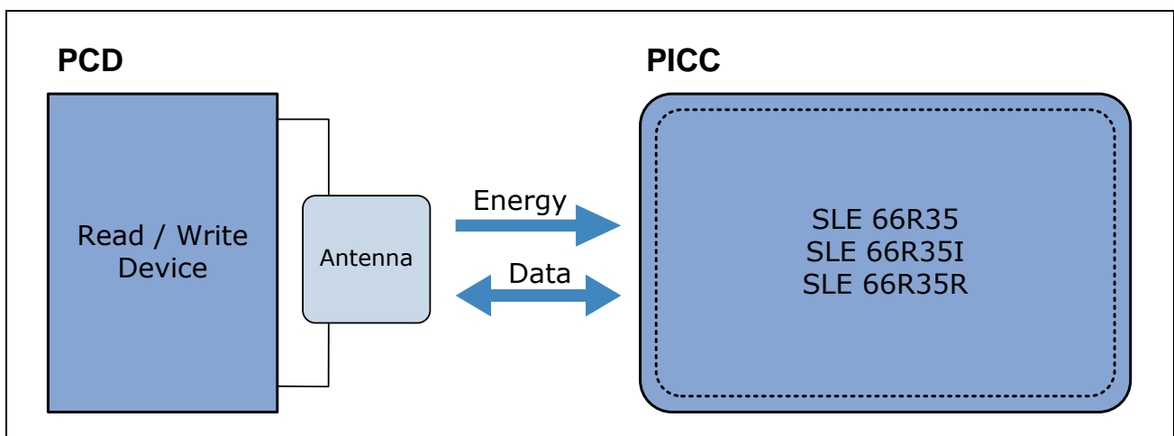
Figure 5 System Overview
