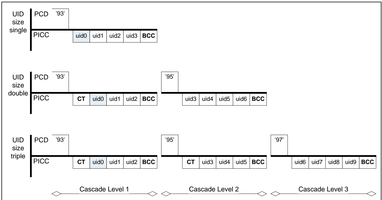
Figure 7 Structures of UID contents and cascade levels according to ISO/IEC 14443-3 Type A
