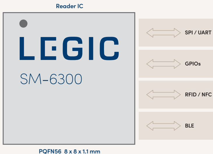
PQFN56 8 x 8 x 1.1 mm
